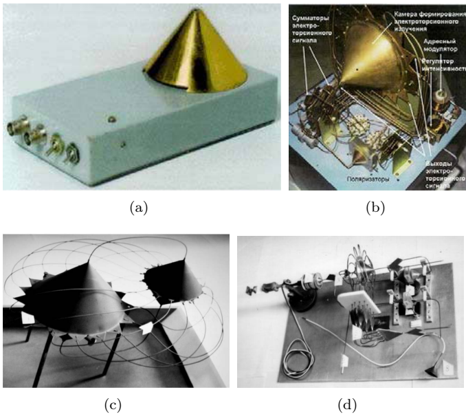
Figure 14. Examples of instrumental generators of a high-penetrating radiation developed at NII MP or under contracts with the center 'Vent': (a,b) small and large Akimov' generators, (c,d) generators of A.Y.Smirnov, images from [97].
