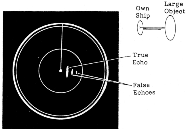
Fig.32 Multiple Echoes
