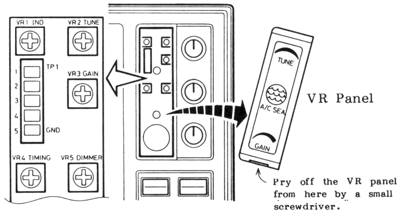
Fig.14 Location of Preset Potentiometers
