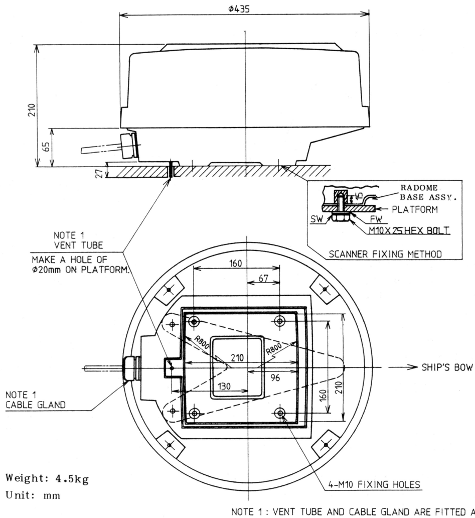
Fig.6 Scanner Unit Outline Drawing
