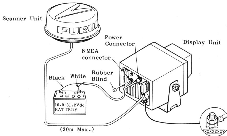
Fig.11 Detailed Wiring Diagram
