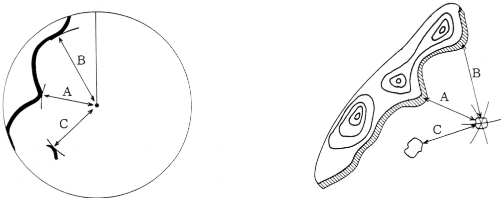
Fig.37 Position Fixing Using Radar Ranges
