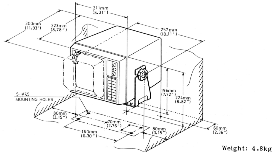
Fig.10 Display Unit Outline Drawing
