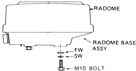
Fig.3 Preparing the Radome Base for Mounting
