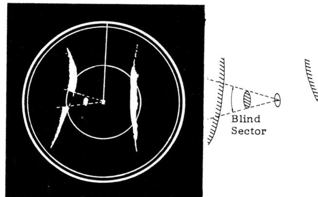
Fig.34 Blind and Shadow Sector
