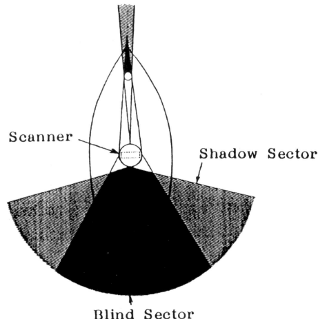
Fig.17 Shadows caused by obstructions
