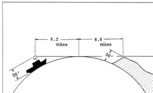
Fig.30 Radar Horizon
