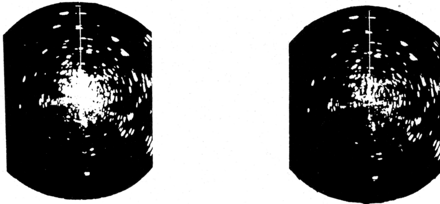
(A) Sea Clutter, A/C SEA control "OFF" (B) A/C SEA properly adjusted
