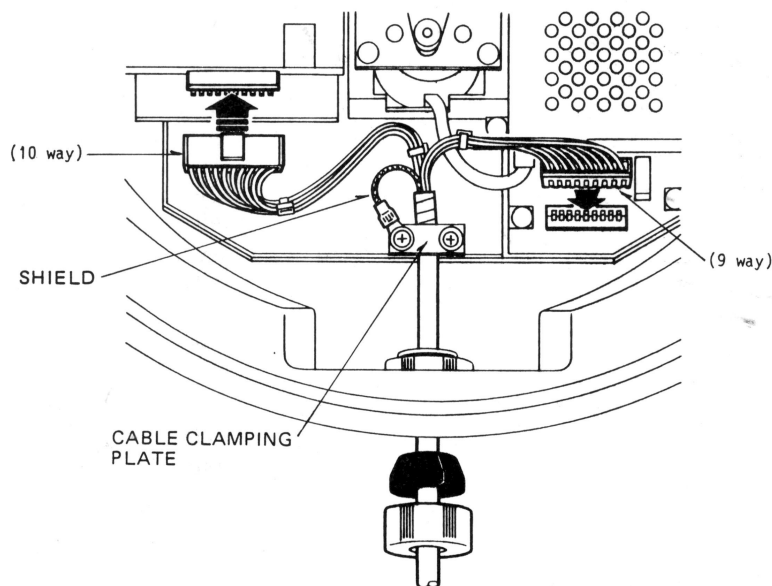
Fig.7 Cable Connection and Grounding
