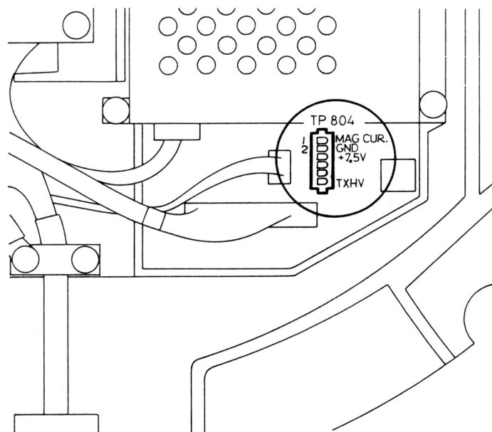
Fig.43 Measuring the Magnetron Current
