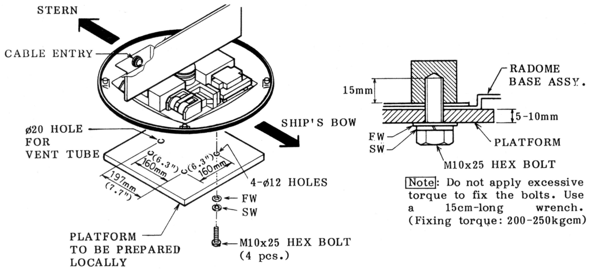
Fig.5 Installing the Scanner Unit
