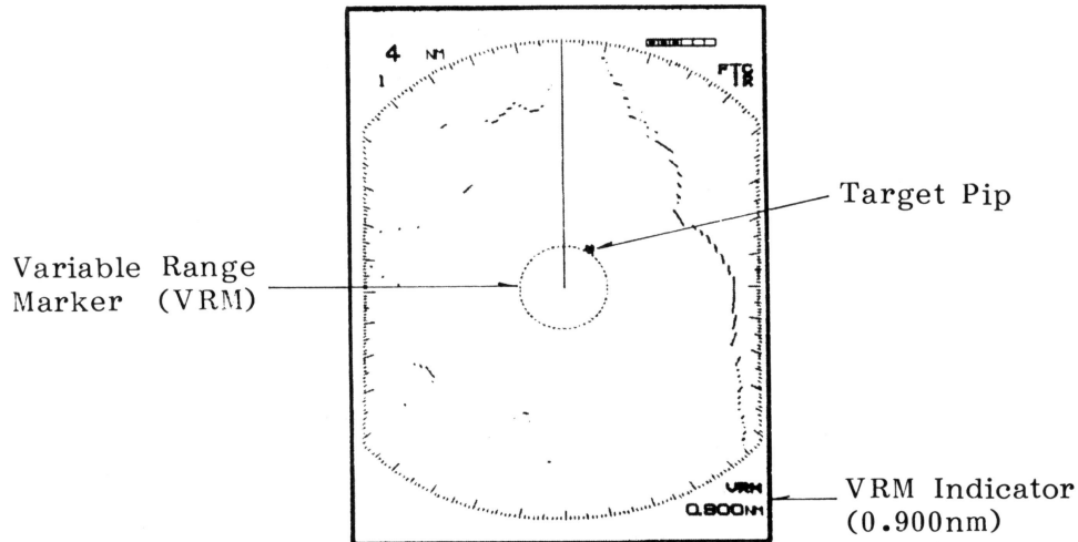
Fig.23 Range Measurement with the VRM Control
