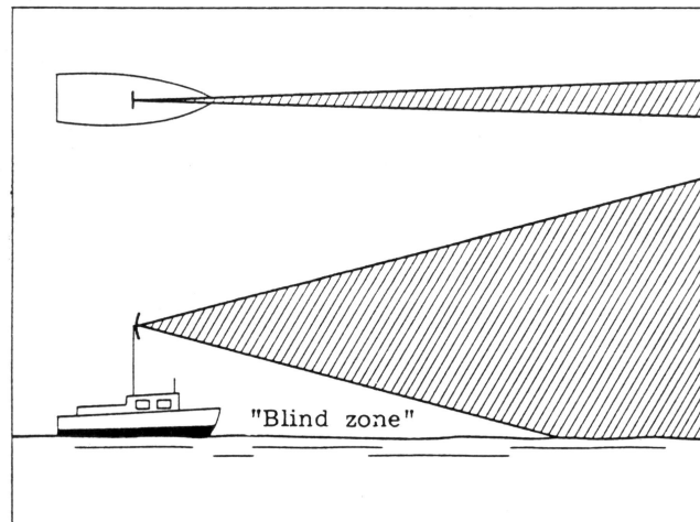
Fig.29 Effects of a Scanner Mounted too High off the Water
