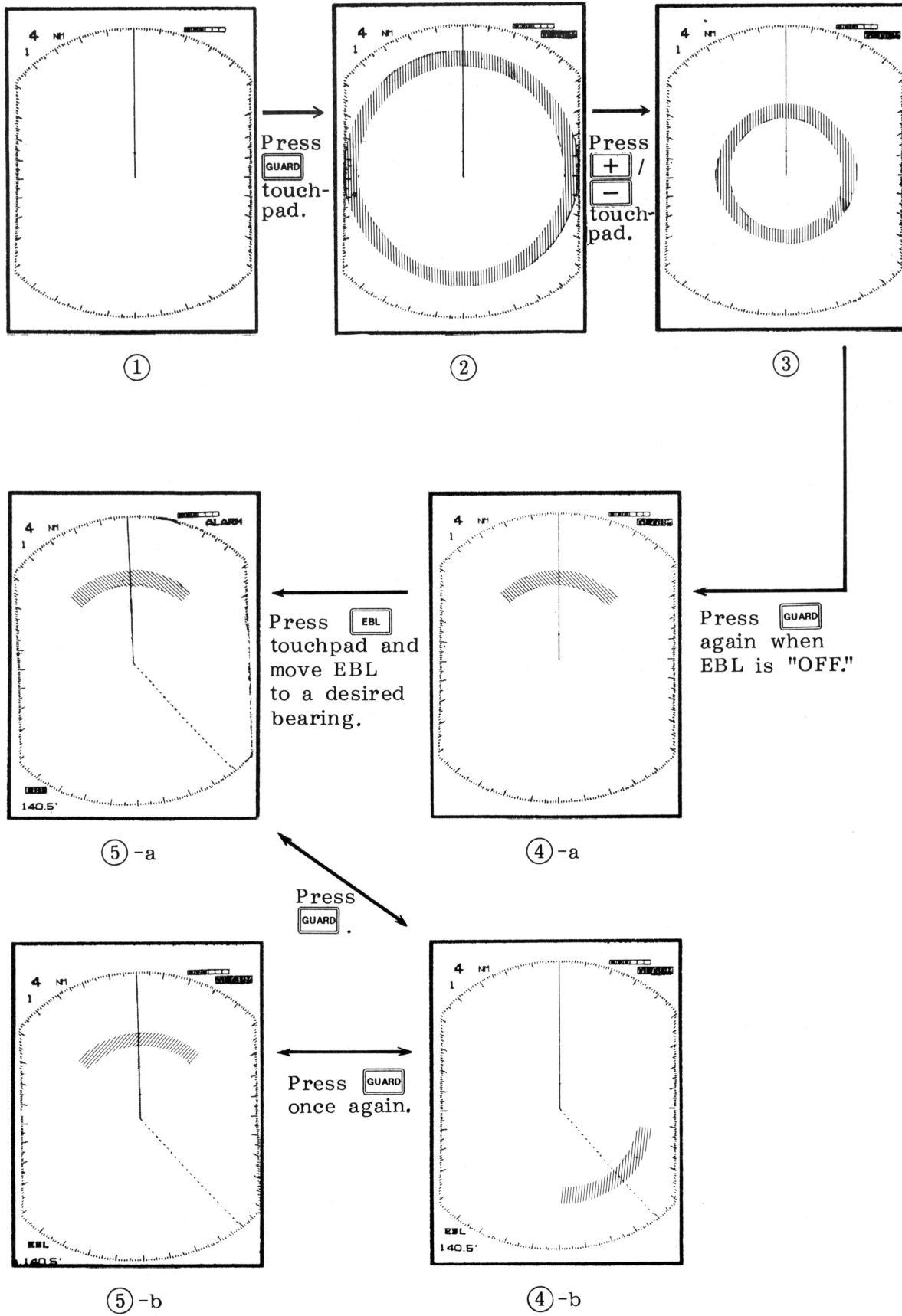
Fig.27 Setting Alarm
