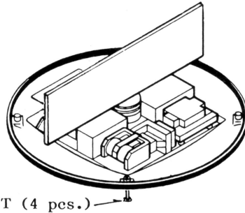
Fig.4 Removing the Radome Cover
