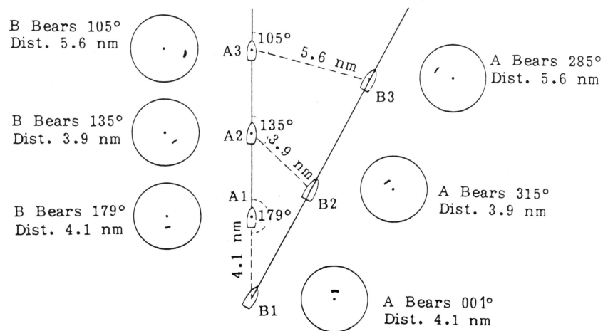
Fig.40 Relative Motion vs. True Motion
