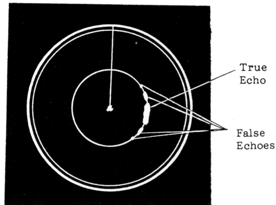
Fig.33 Side-Lobe Echoes
