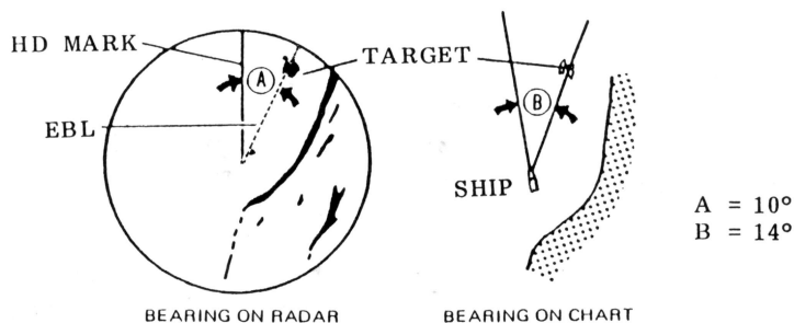
Fig.12 Relative Bearing Alignment
