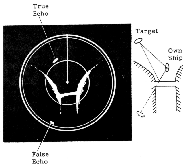
Fig.35 Indirect Echoes
