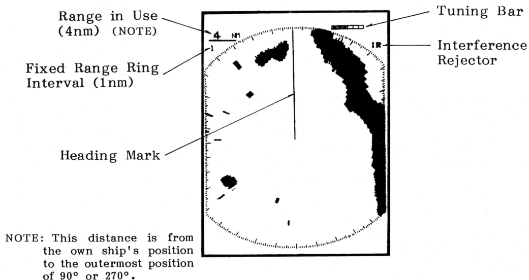
Fig.20 Location of Display Screen Indicators
