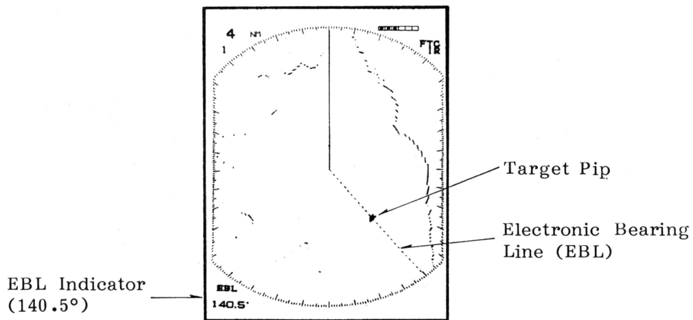
Fig.24 Measuring the Bearing of a Target Pip with the EBL
