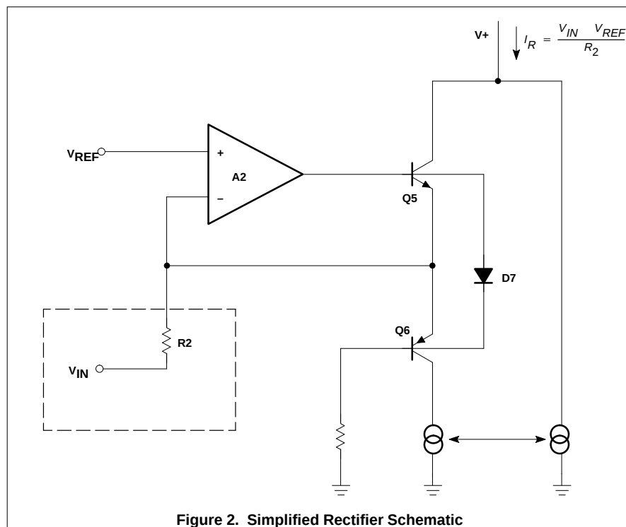
Figure 2. Simplified Rectifier Schematic
