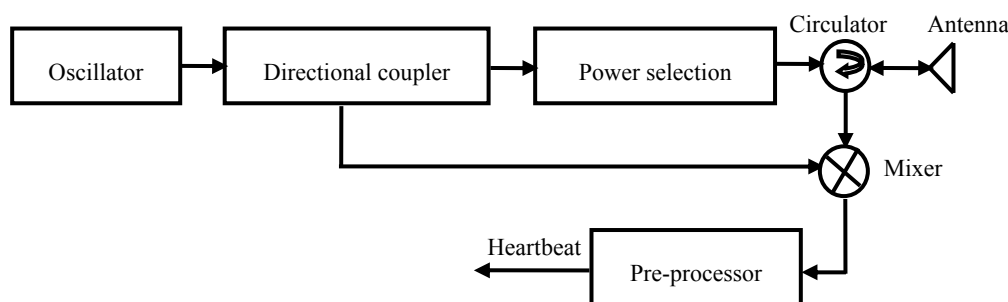
Figure 1. The block scheme of the microwave sensor.
