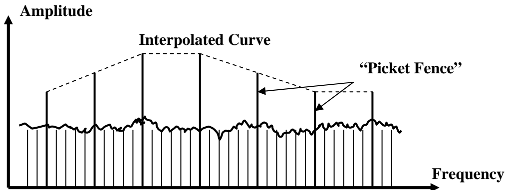
Figure 5. Display of “tracked” frequency measurement using the DSI Technique
