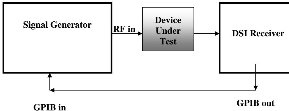
Figure 3. Swept frequency tracking with a DSI Receiver
