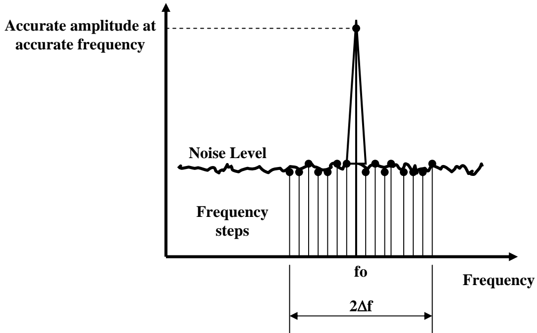
Figure 4. The DSI technique for cheap frequency “tracking” measurements
