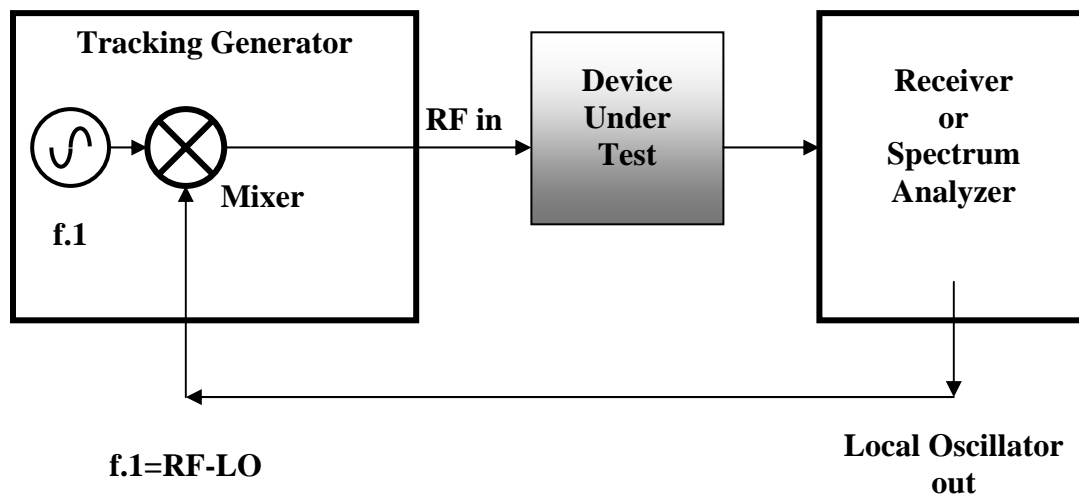
Figure 1. Basic setup for swept frequency measurement using a tracking signal generator
