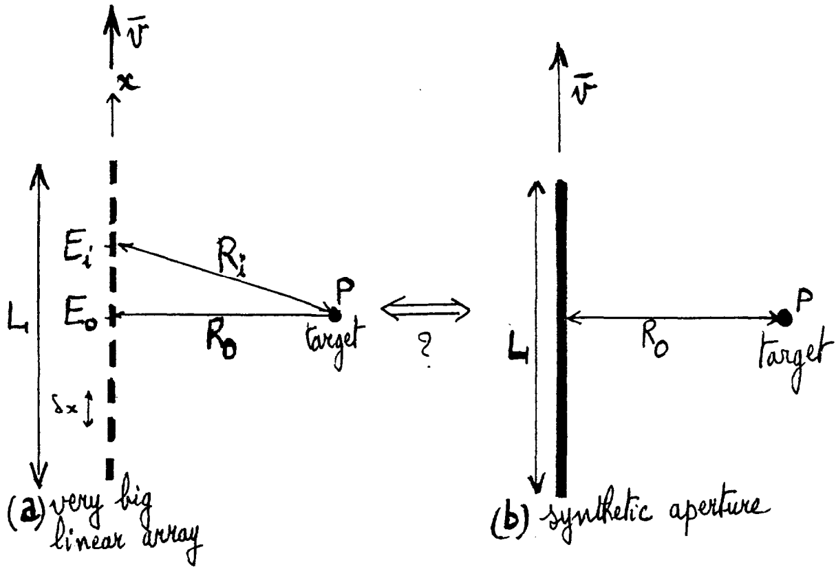
Fig. B9. Very big linear array and corresponding synthetic aperture of aperture length L
