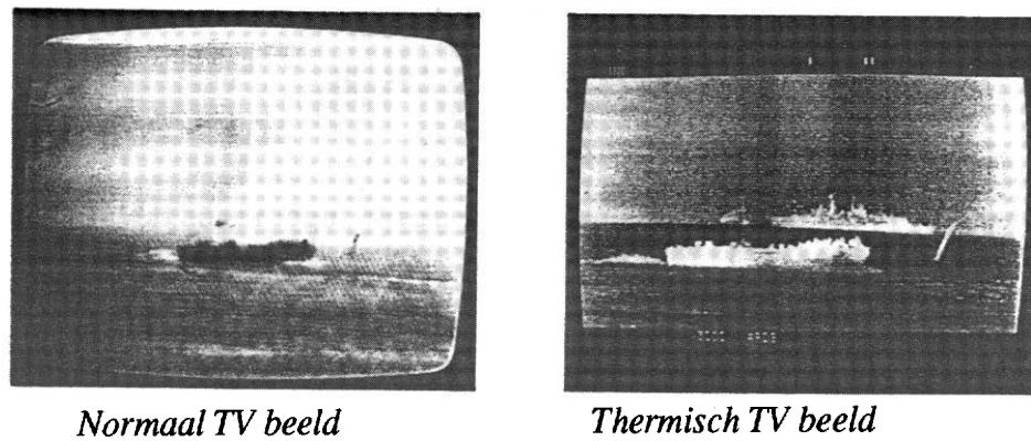
Fig.A2. ( Visible ) TV image (left) and thermal image (right) taken with a Th IR camera in the ( 8\mu\text{m}-12\mu\text{m} ) band on a hazy day in Den helder ( NL ). On the lefthand "visible" image, one ship is barely distinguishable at a few hundred meters from the pier. On the ( righthand ) thermal image a second vessel is clearly visible at 6km from the pier.
