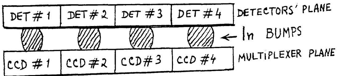
Fig.A20. Hybrid integration for InSb and CMT detectors
