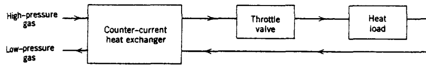
(a) Schematic of Cryostat Operation
