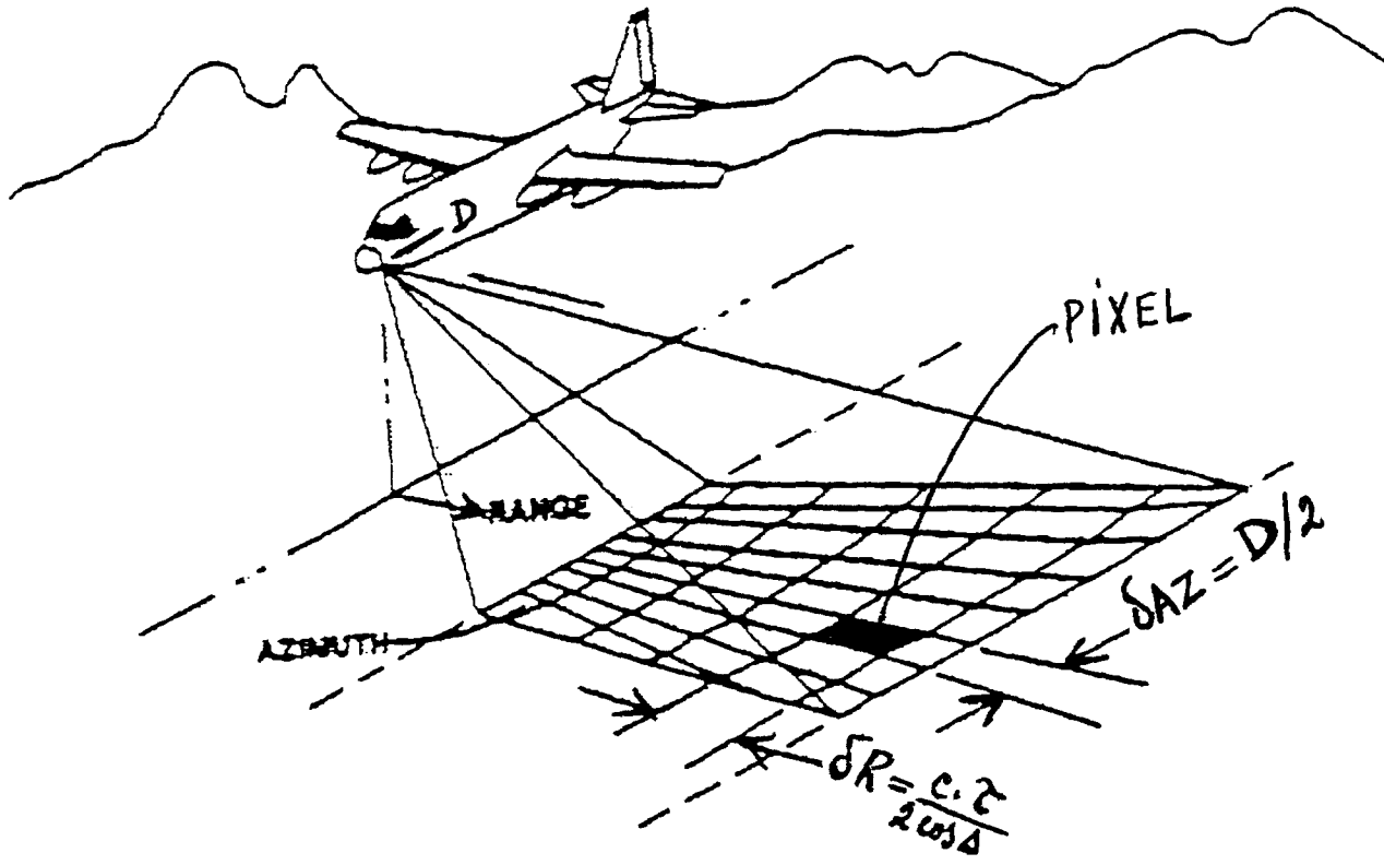
Fig. B12. SAR pixel
