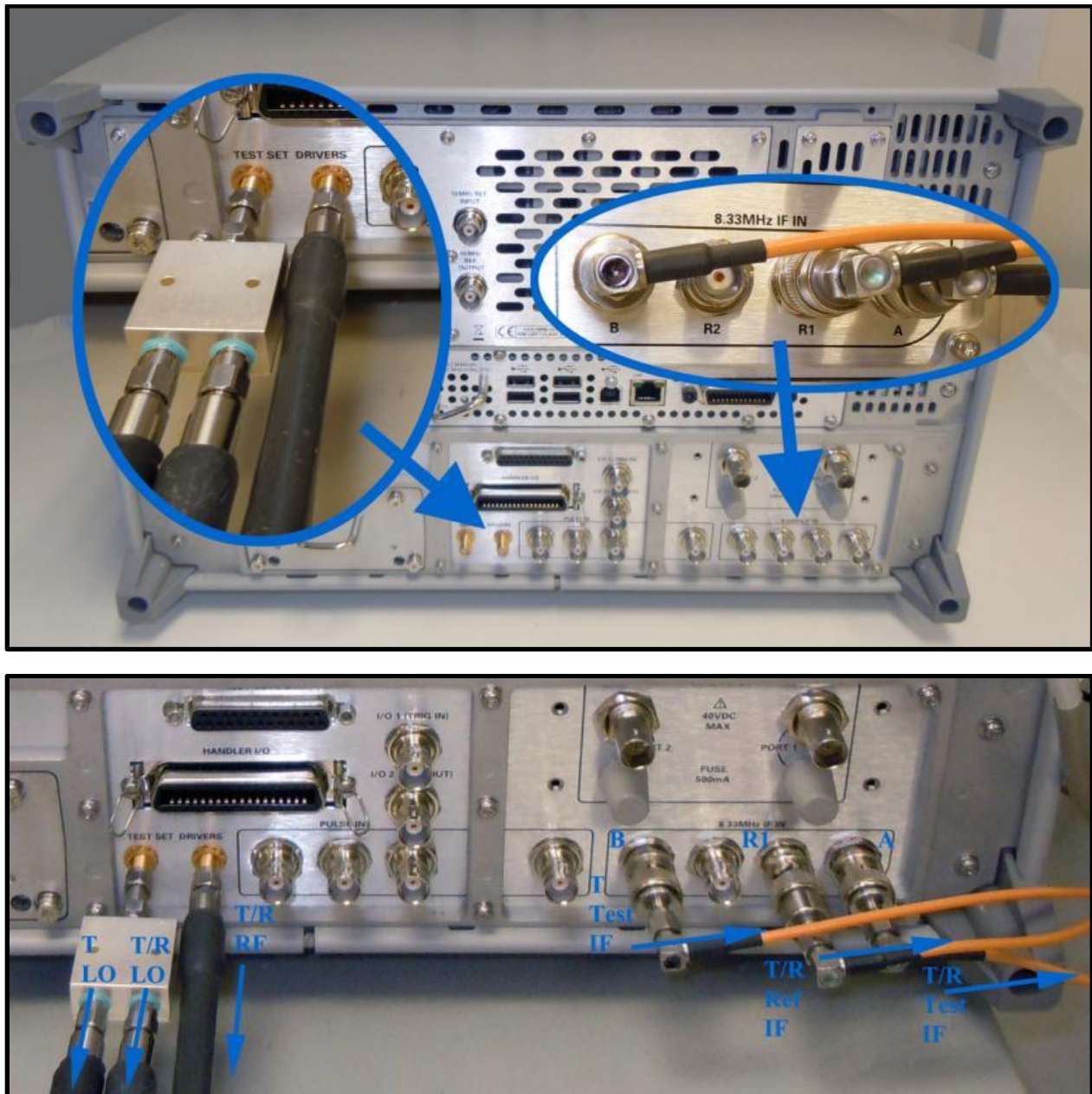
Figure 2. Shown is the rear view (including close-ups) of the overall millimeter wave setup consisting of Agilent's PNA, OML's VNA extension modules, and interconnects. Note that this setup does not include the N526xA millimeter-wave controller. On the left, phase-stable RF cables are connected to the Test Set Drivers output; the LO is split as shown. On the right, the IF cables are connected as shown to access the PNA's receivers for S11 and S21 measurements.
