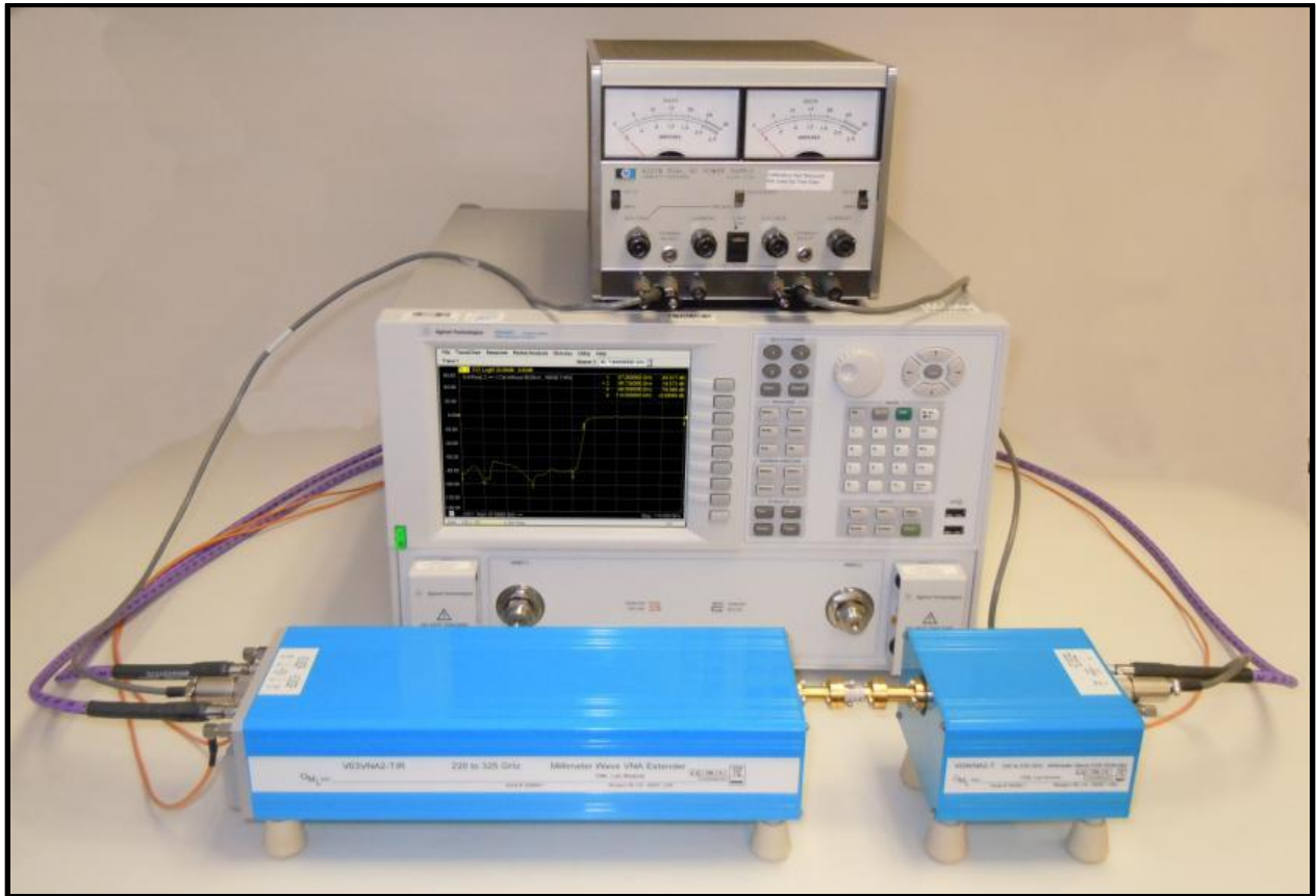
Figure 1. Shown is the front view of the overall millimeter wave setup consisting of Agilent's PNA, OML's VNA extension modules, power supply, and interconnects. Note that this setup does not include the N526xA millimeter-wave controller. Left to right, OML T/R and T modules are shown with a through connection. The RF, LO, and IF signals are connected to the rear panel of the PNA. In this configuration, the setup supports enhanced calibrations for S_{11} and S_{21} measurements.
