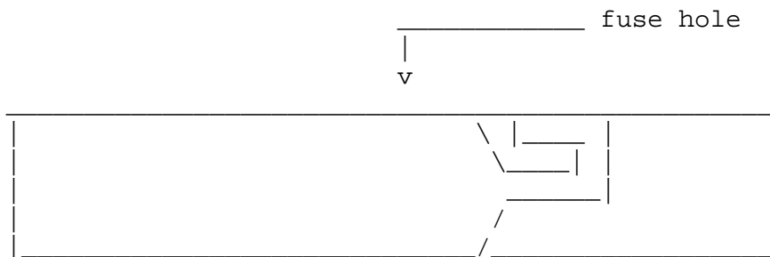
fig. 3 pipe with flattened and folded end (side view)
