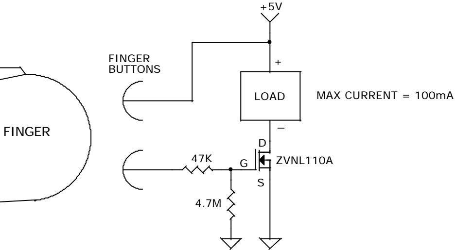
ELECTRICAL CONDUCTION THROUGH FINGER TURNS ON THE MOSFET
