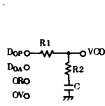
Passive filter
