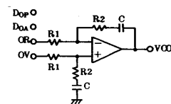
Differential filter
