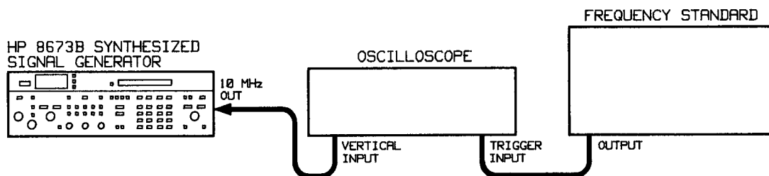
Figure 4-11. Internal Time Base Aging Rate Test Setup
