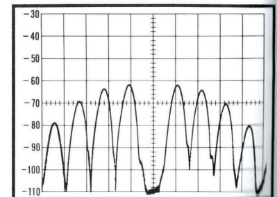
Deep null appears at exactly 5 kHz
